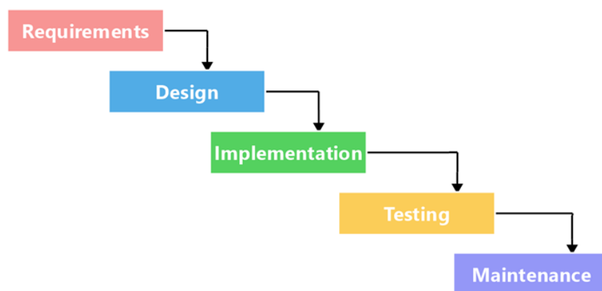
Figure. 1 Waterfall Model
