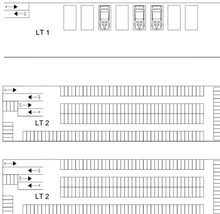
Figure 6. Parking Building Layout Segment 1
