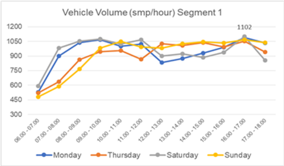
Figure 11 Vehicle Volume
