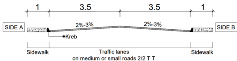
Figure 4. Cross-section of Segment 2
