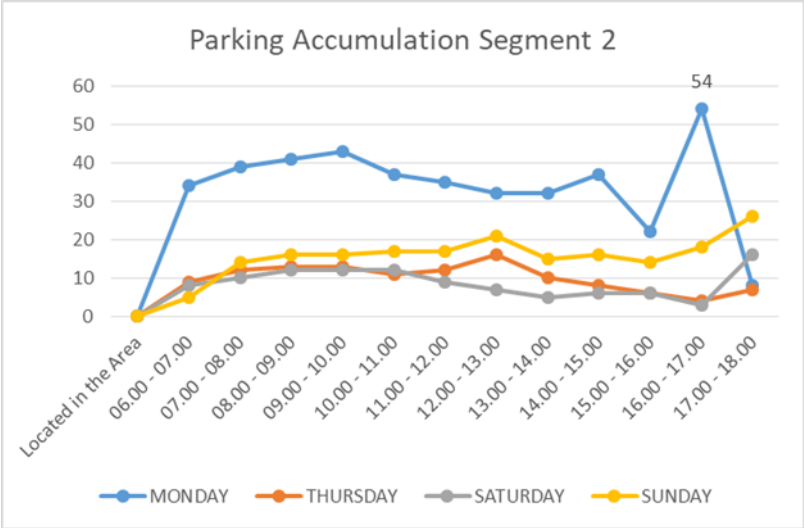
Figure 5. Segment 2 Parking Accumulation
