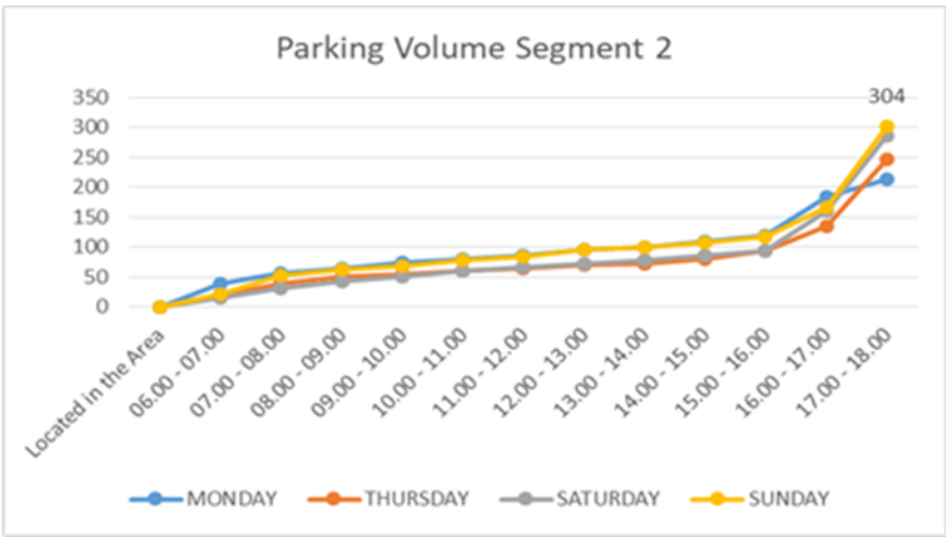
Figure 7. Segment 2 Parking Volume
