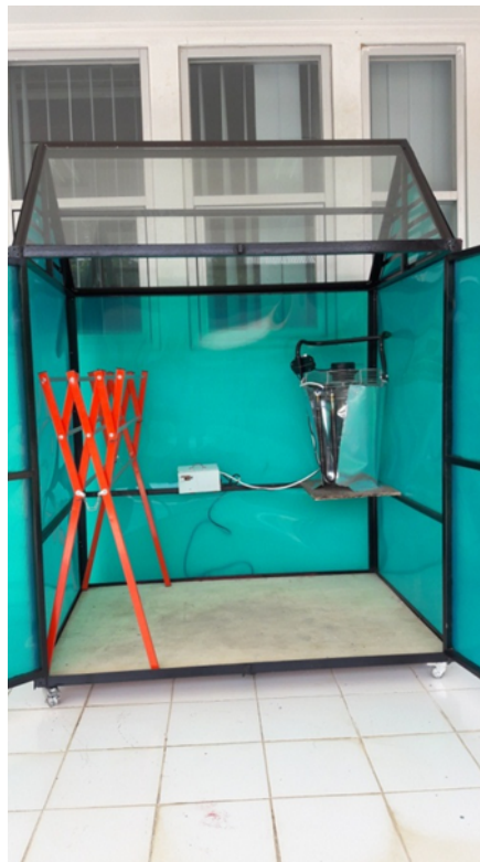
Figure 4. Deep Visible Automatic Clothes Drying Chamber
