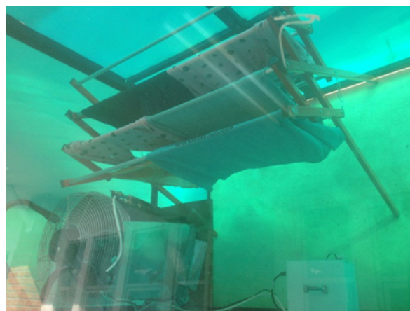
Figure 3. Top View Automatic Clothes Drying Chamber
