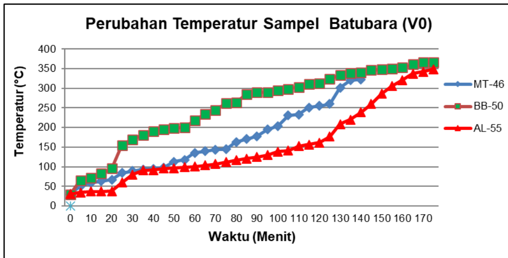
Figure 7. Coal Transition Temperature of 50 mm at No Wind Speed (V0)
