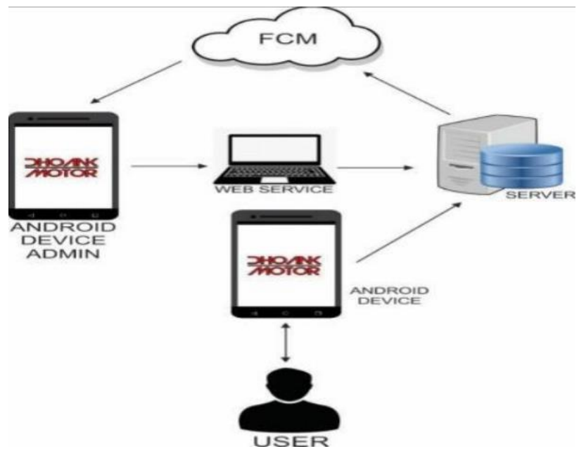
Figure 2 Model Architecture
