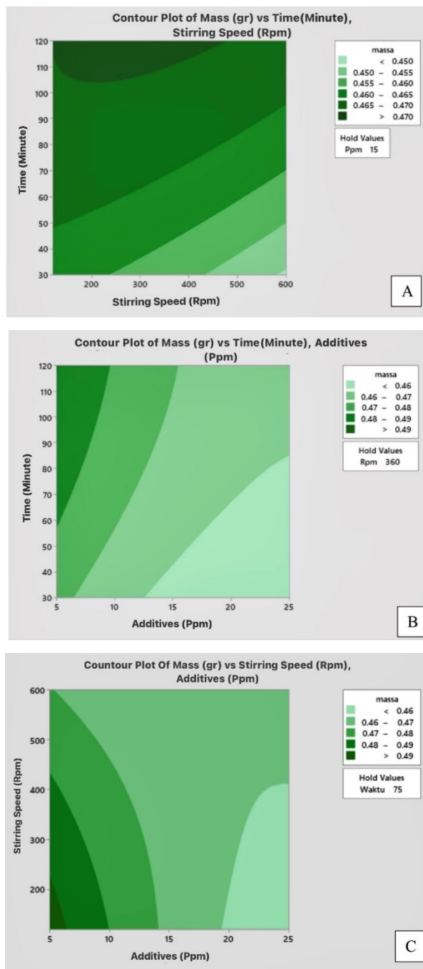
Figure 3 Contour optimization area of the recovery of barium sulfate crystals (a) variable stirring speed and stirring time (b) variable concentration of \text{FeCl}_2 additive and stirring time (c) the variable concentration of the \text{FeCl}_2 additive and stirring speed
