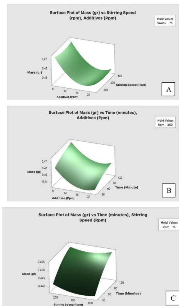
Figure 6 Surface plot of the optimization area of the recovery of barium sulfate crystals (a) variable concentration of \text{SrCl}_2 additives and stirring speed (b) variable concentration of \text{SrCl}_2 additives and stirring time (c) variables of stirring speed and stirring time
