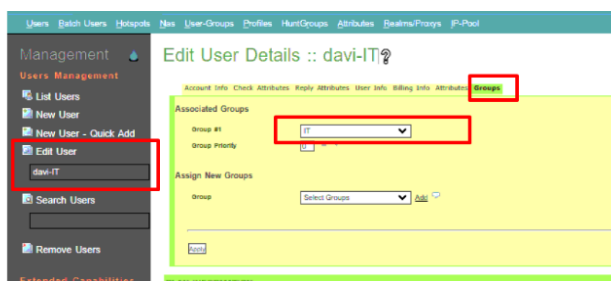
Figure 9 Grouping Management dalorRADIUS
