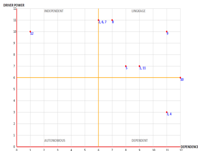
Figure 1 Micmac Model
