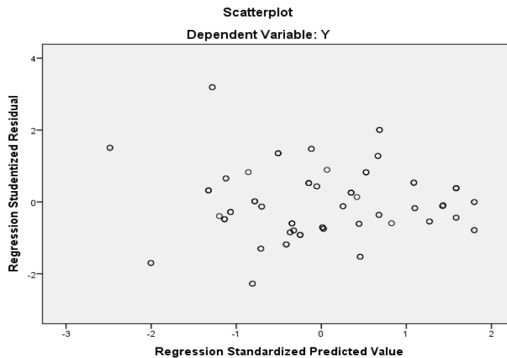
Figure 3 Scatterplot Results
