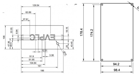
Figure 2. Front and Rear View Sketch of EVPLC
