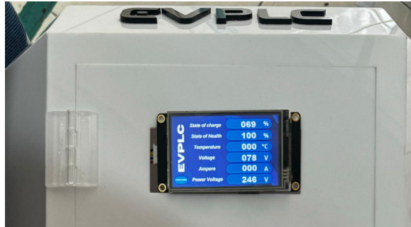
Figure 18. HMI of EVCS Demo Module
