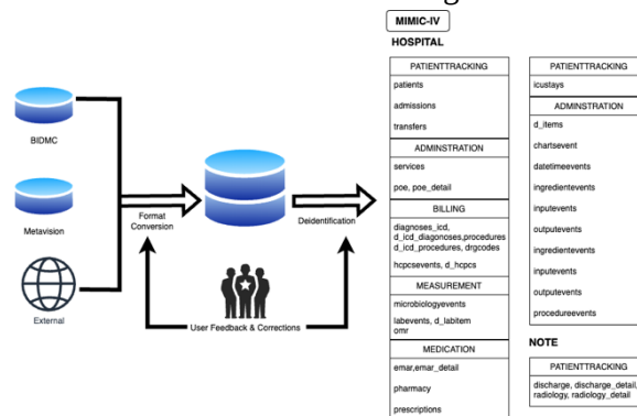
Figure 1. Dataset Structure
