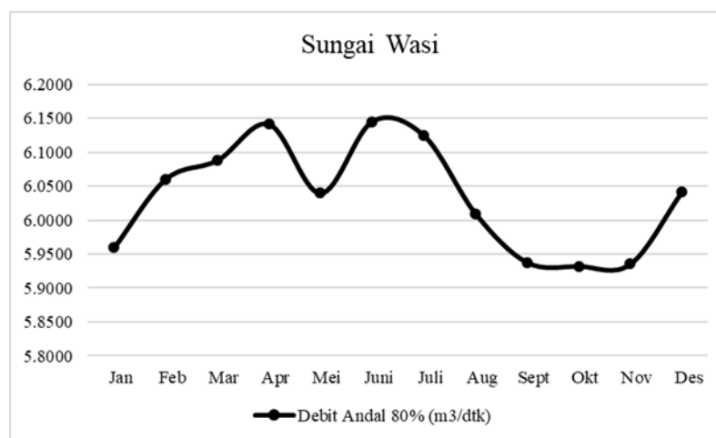
Figure 1 Reliable Discharge (Q80) of the Wasi River
