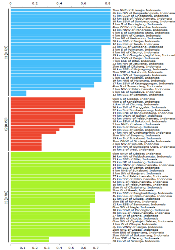
Figure 6 Clustering Results
