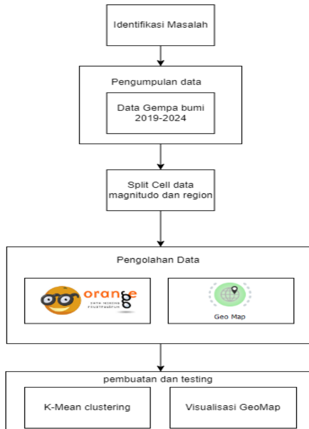
Figure 1 Research Methods
