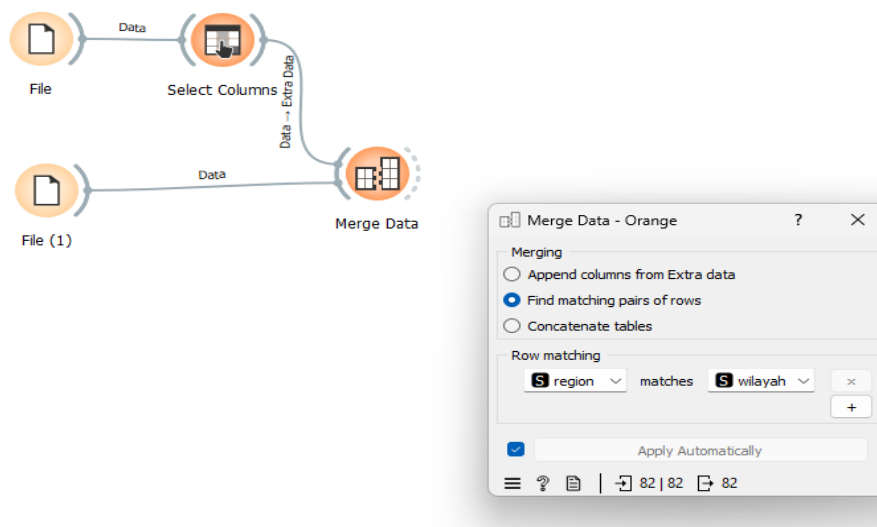
Figure 5 Merge Data
