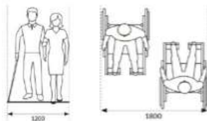
Figure 1. Circulation Width Dimension
