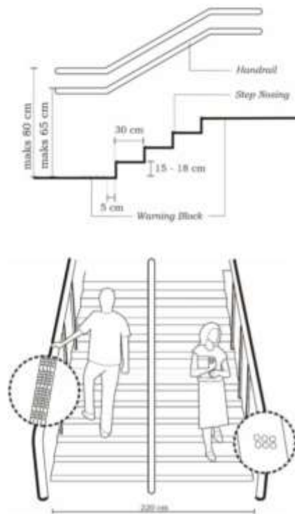
Figure 2. Standard Size of Stairs
